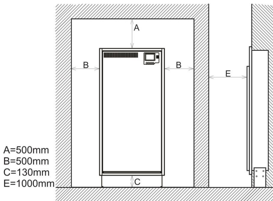
Minimum dimensions of free mounting space
