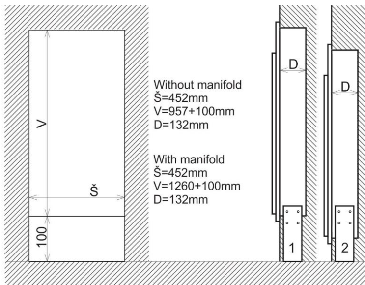
Minimum dimensions of free mounting space
